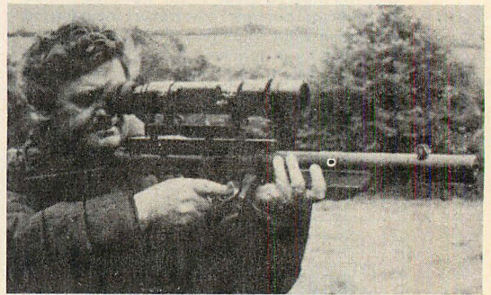
Scotos I/RS unit on L34A1 (silenced Sterling) 9mm SMG.
